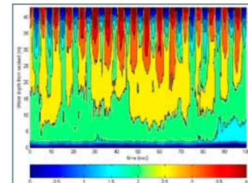
The image above visualises outputs from a Tidal Bladed simulation of extreme waves in a turbulent flow
